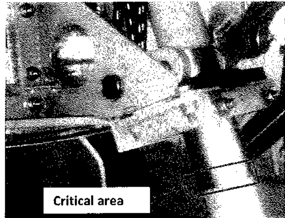
B, Nose gear leg with reinforcement
